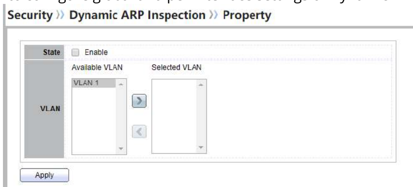
Figure 10-33 Property Page
