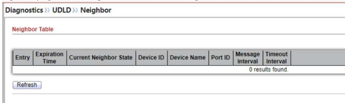
Figure 13-12: Neighbor page.
