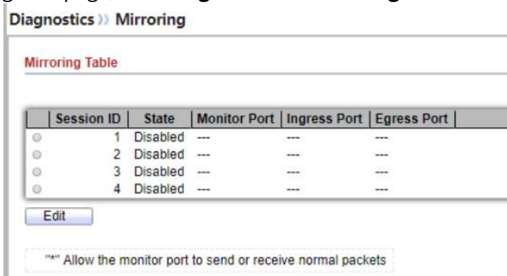
Figure 13-3 Mirroring Page
