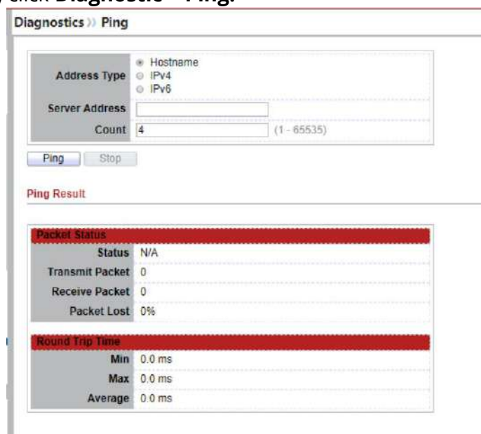
Figure 13-4: Ping page.
