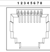
Figure 1 10/100/1000M Lan Port Pinouts
