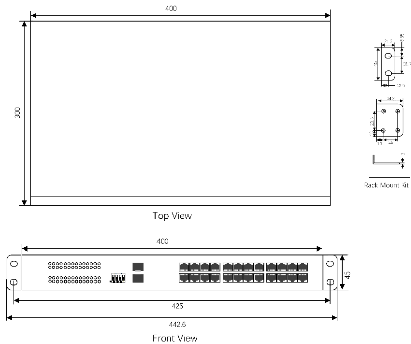
24x10/100/1000Base-TX RJ45+2x1000Base-X SFP
