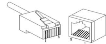
Figure 1 10/100/1000M Lan Port Pinouts
