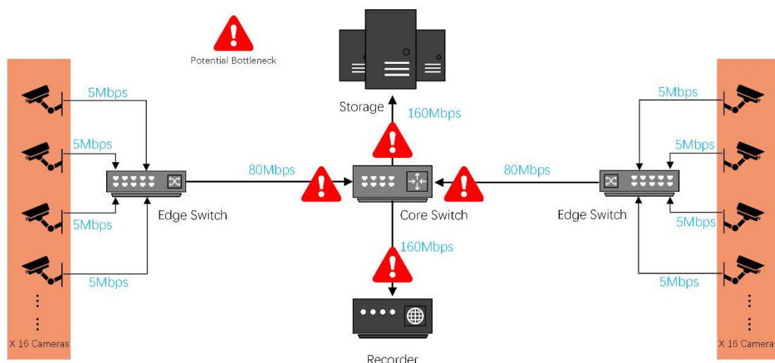
Figure 6: Bandwidth bottlenecks
