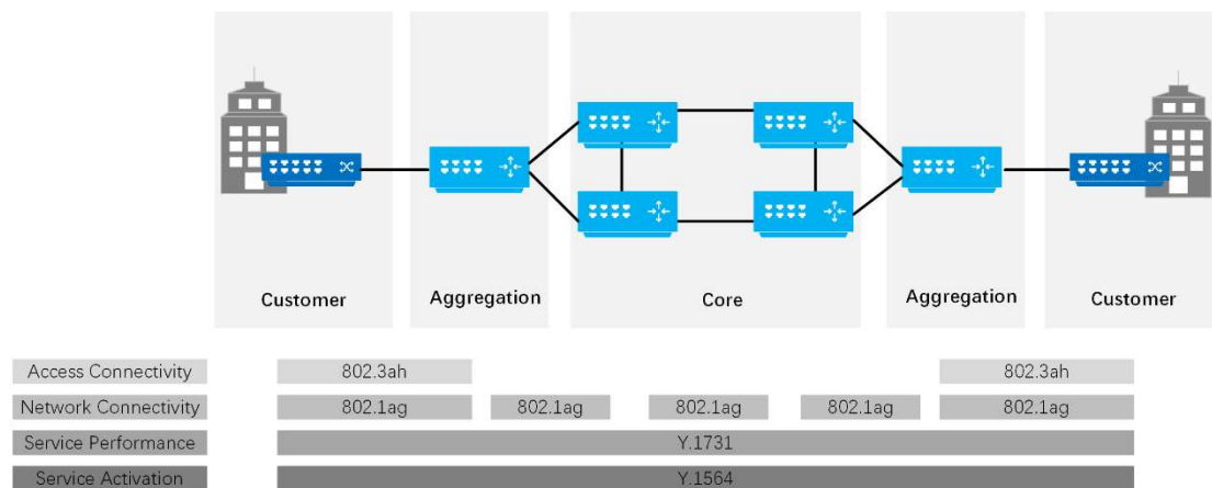
Figure 1 Typical MAN Networking
